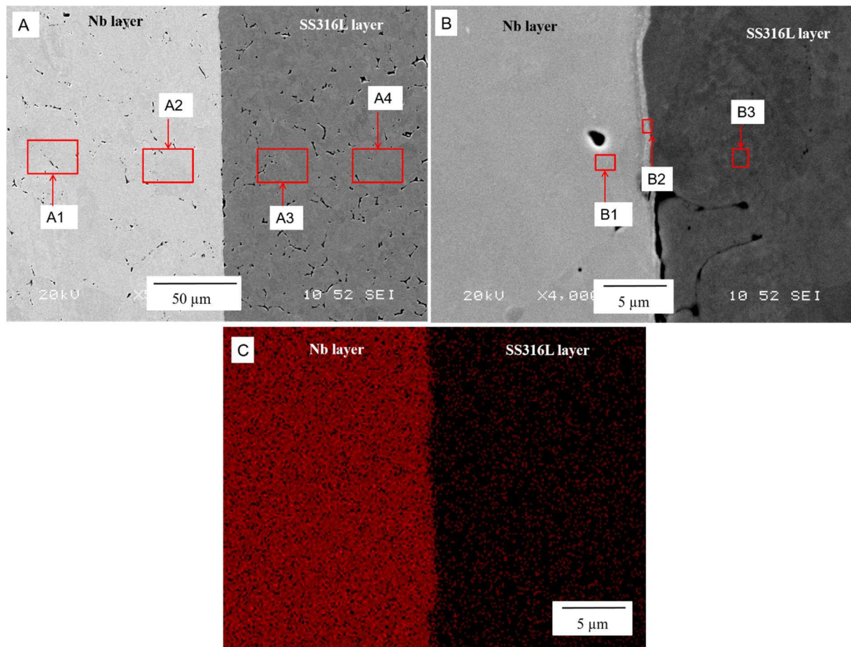
Figure 8. (a, b) SEM images of the cross-section of SS316L/Nb composite produced by FAST/SPS. Nb layer was consolidated at 1500 °C and SS316L layer at 1000 °C. (c) EDS mapping of Nb.
