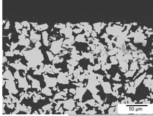
Figure 2. SEM image of Ti-PTL used as reference samples.
